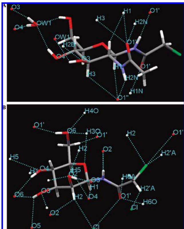
Figure 7. Representation of the hydrogen bonds and interaction network in the crystalline environment of GlcNAc \beta NHCOCH 2 Cl ( 3 ), above, and Man \beta NHCOCH 2 Cl ( 6 ), below.
