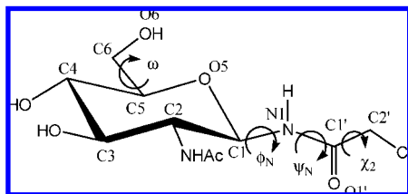
Figure 1. Schematic representation of GlcNAc \beta NHCOCH 2 Cl together with the various torsion angles of interest \phi_N = \text{O5-C1-N1-C1}' , \psi_N = \text{C1-N1-C1}'\text{-C2}' , \omega = \text{O5-C5-C6-O6} , and \chi_2 = \text{N1-C1}'\text{-C2}'\text{-C1} .
